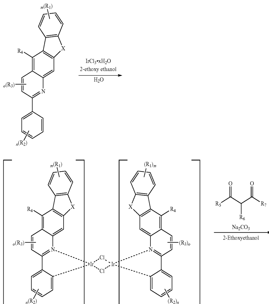
[Reaction Scheme 1]
